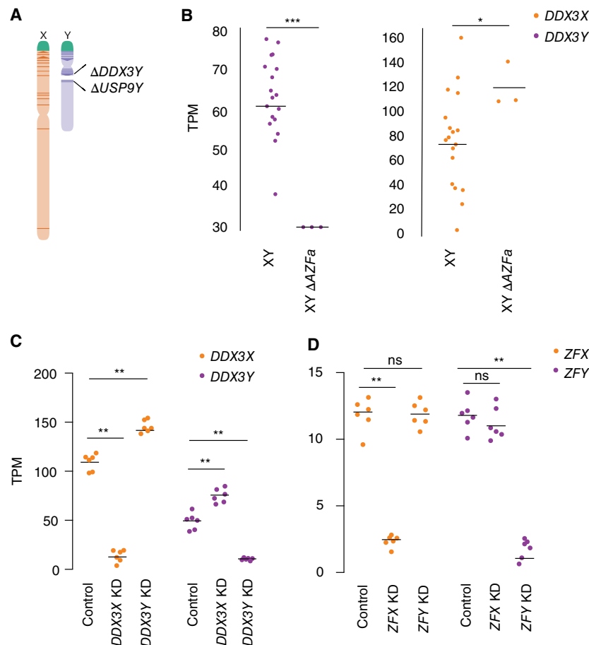
Figure 3. DDX3X and DDX3Y each respond to perturbations in the other's expression. (A) Schematic diagram of naturally occurring Chr Y (AZFa) microdeletion of DDX3Y and USP9Y . (B) DDX3X transcript levels are significantly higher in AZFa-deleted 46,XY LCLs compared with 46,XY LCLs with intact Chr Y. Each point represents a sample from one individual. Statistical significance determined by Mann–Whitney U-test: (***) P < 0.0001 , (*) P < 0.05 . (C) CRISPRi-mediated knockdown of DDX3Y using two independent gRNAs in three unrelated 46,XY fibroblast cultures results in significantly elevated DDX3X transcript levels. Conversely, DDX3X knockdown results in significantly elevated DDX3Y transcript levels. (D) Reanalysis of CRISPRi knockdown of ZFX or ZFY (San Roman et al. 2024) demonstrates that knockdown of either gene does not result in significant elevation of the homolog's transcripts. Statistical significance determined by ANOVA: (**) P < 0.001 .
