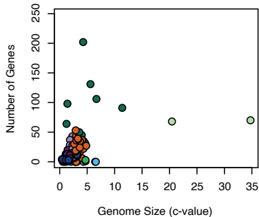
All Vertebrates
