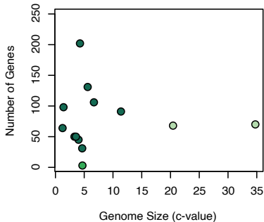
Amphibians only
