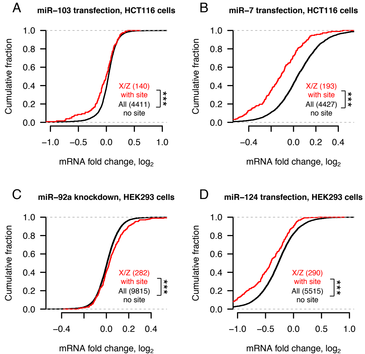
Supplemental Figure S17: Gene expression changes following transfection or knockdown of additional miRNAs in human HCT116 or HEK293 cells. *** p < 0.001 , two-sided Kolmogorov-Smirnov test.
